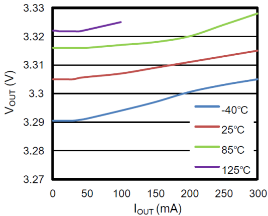
11. V_{OUT-I_{OUT}} vs. Temperature
