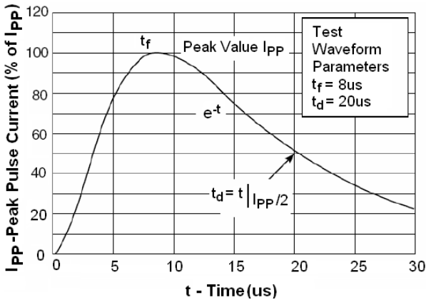
Figure1. Pulse Waveform
