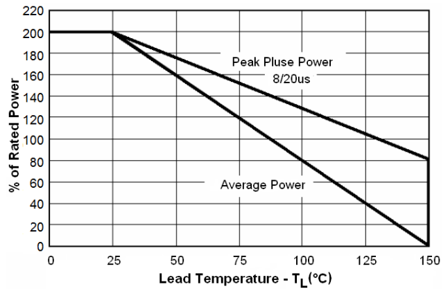
Figure 2. Power Derating
