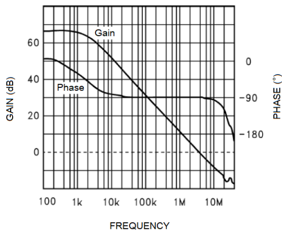
34. Gain/ Phase Response, A_v=2 V_{DD}=5V , 8\Omega Load, C_{LOAD}=500pF
