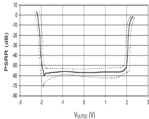
23. PSRR vs. DC Output Voltage V_{DD}=3V , A_v=10
