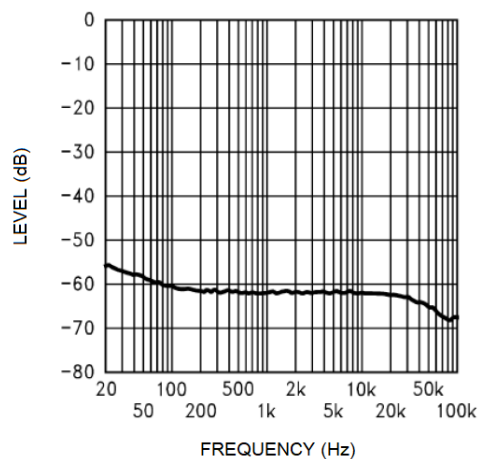
16. Power Supply Rejection Ratio (PSRR) @ A_V=4 , V_{DD}=3V , V_{ripple}=200mVp-p , R_L=8\Omega , R_{IN}=10\Omega
