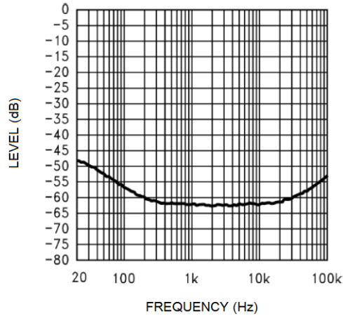
14. Power Supply Rejection Ratio (PSRR) @ A_V=2 , V_{DD}=3V , V_{ripple}=200mVp-p , R_L=8\Omega , R_{IN}=10\Omega
