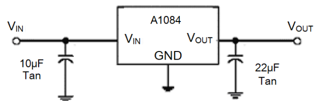
Fig 1. A1084 fixed version application circuit
