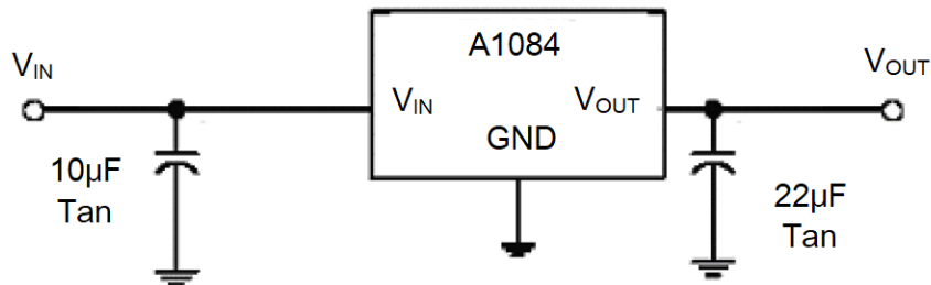
Fig 1. Typical Application of A1084
