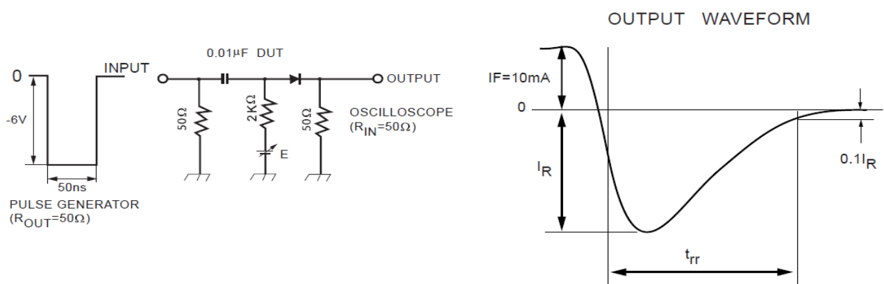
Figure 5. Reverse recovery time ( t_{RR} ) test circuit
